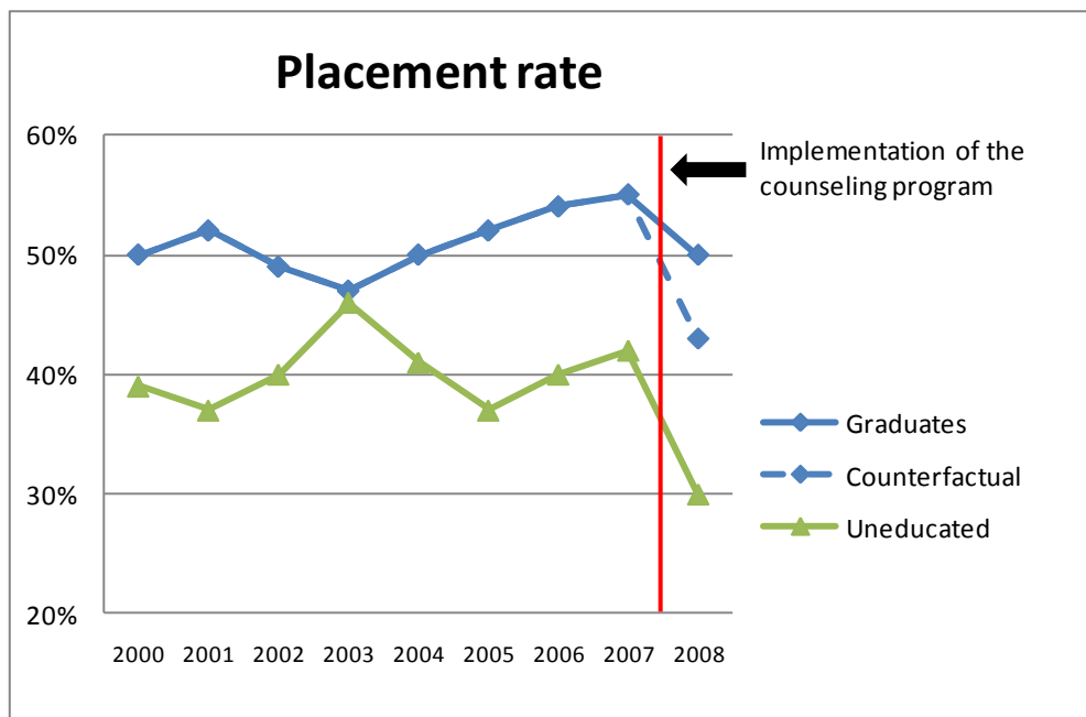
Figure 6: A graph contradicting the parallel trend assumption
