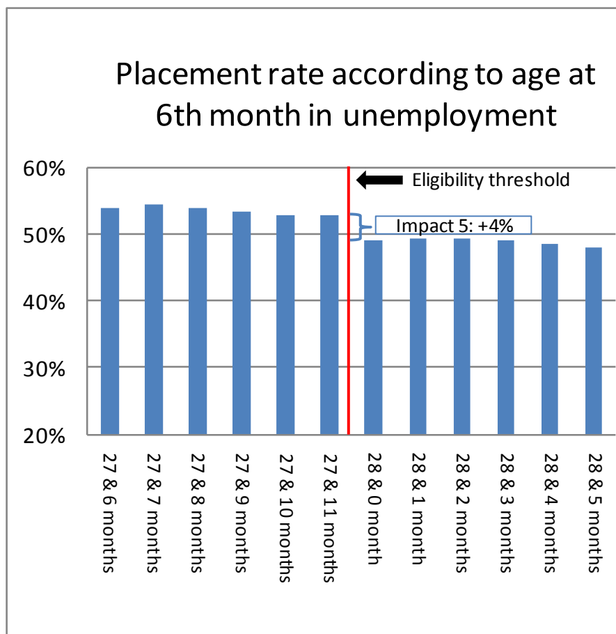
Figure 7: A graph supporting the regression discontinuity approach
