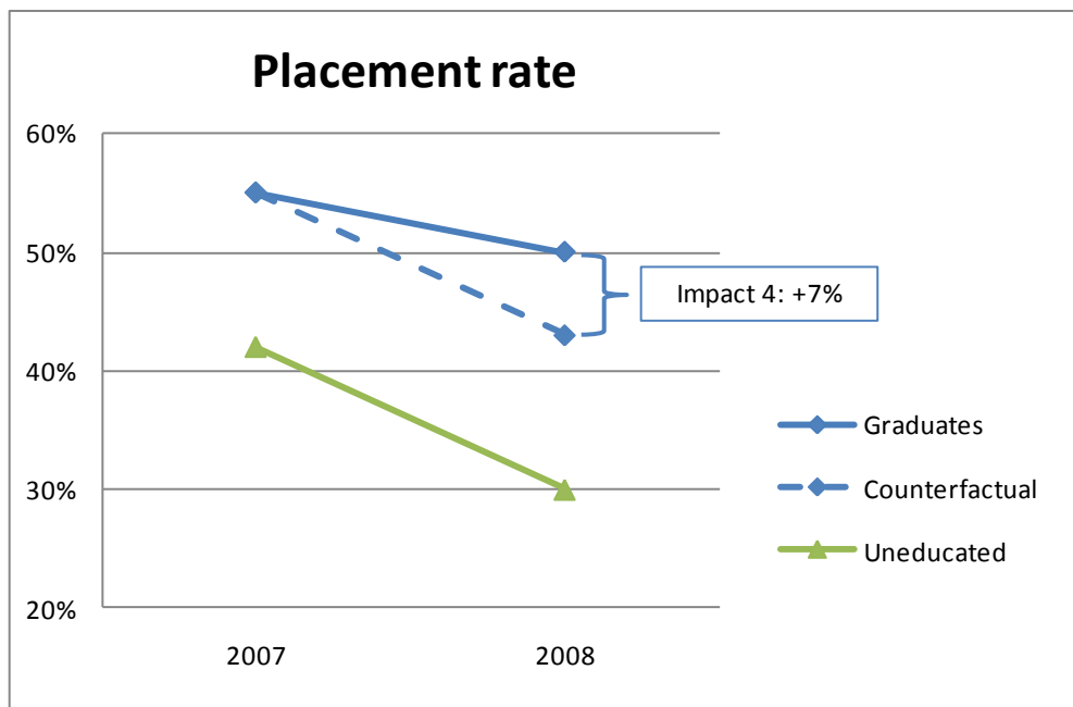
Figure 4 : Difference in differences
